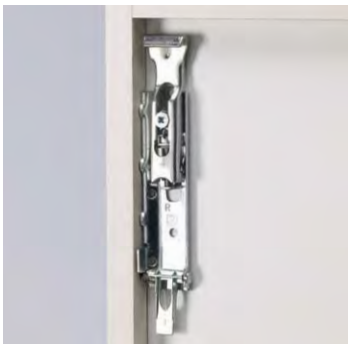
Fig. 1 Adjustable wall hanging bracket.
